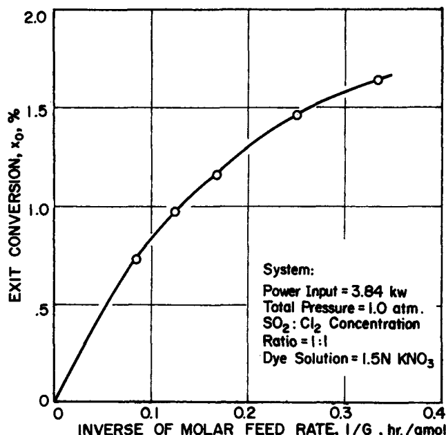
Fig. 2. Exit conversion of sulfur dioxide vs. the inverse of the molar feed rate.
